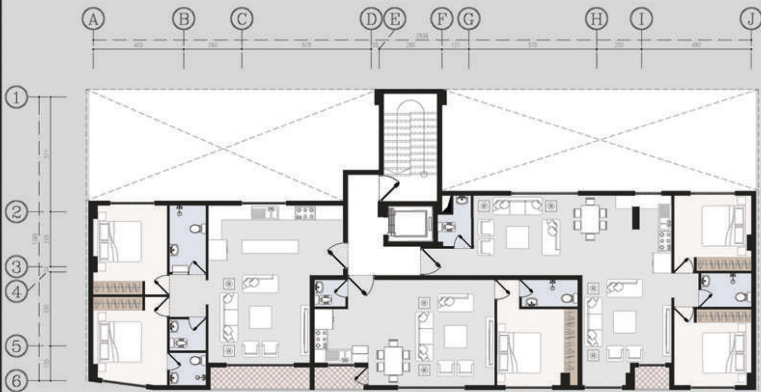
Typical Plan
